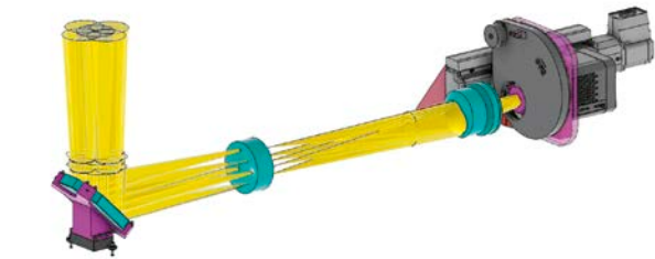
TARSIS instrument acquisition and guiding system design
