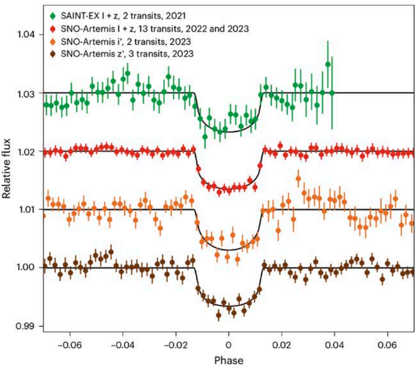
Fig. 1. Discovery transit photometry of SPECULOOS-3 b, an Earth-sized exoplanet orbiting the nearby ultracool dwarf star SPECULOOS-3. Data obtained by SAINT-EX and SNO-Artemis between 2021 and 2023 at different filters. For clarity, the light curves are shifted along the y-axis. Figure from [148].
