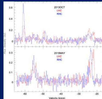
Spectra of circular polarization of the OH emission at 1720 MHz from the PN IRAS 16333-4807, showing Zeeman splitting in the line (shift between the two circular polarizations)
