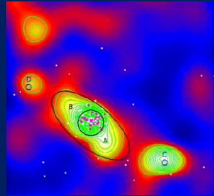
Galaxy density map in the cluster LCDCS 0829 ( z = 0.4510 ). The large black circle shows 1 Mpc around the cluster center. The (C,D) circles correspond to galaxy clusters in NED
