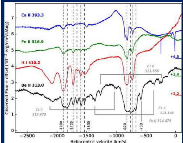
Be absorption in the spectra of nova V5668Sgr at 82
