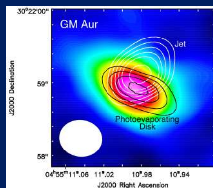
Image of the dust and ionised components in the young star GM Aur. The disc of dust is shown in colour scale, the ionised jet in white contours, and the ionised photoevaporative wind arising from the disc in black contours
