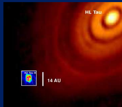
A comparison (same scale) of the size of the well-known protoplanetary disc around HL Tau and the dwarf disc around XZ Tau
