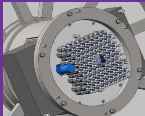
Layout of the focal plane of MEGARA with the 92 robotic positioners
