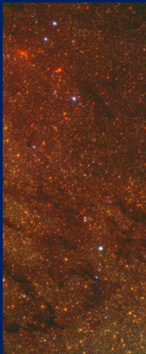
RGB image of a field in the Galactic Centre based on JHK data taken with HAWK-I/VLT as part of the GALACTICNUCLEUS survey. The field of view is about 8 arcmin by 3 arcmin with an angular resolution of 0.2
