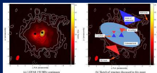
The LOw Frequency ARray (LOFAR) unveils kpc-extended disks surrounding the nuclei of the closest ULIRG, Arp220
