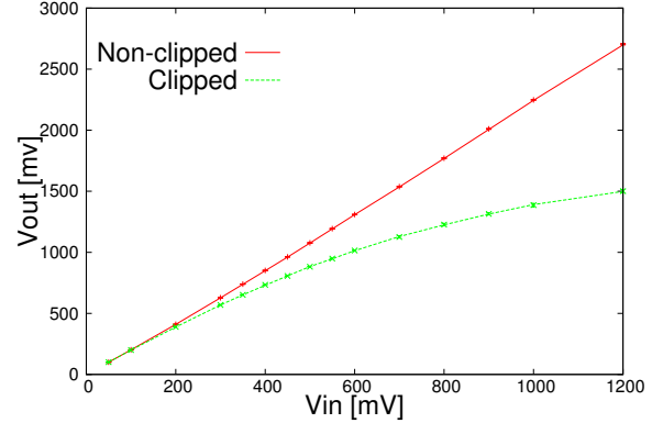
Figure 3.13: Transfer function of the analog discrete component trigger where the clipping is applied. In red we show the non-clipped signal and in green the clipped one.
