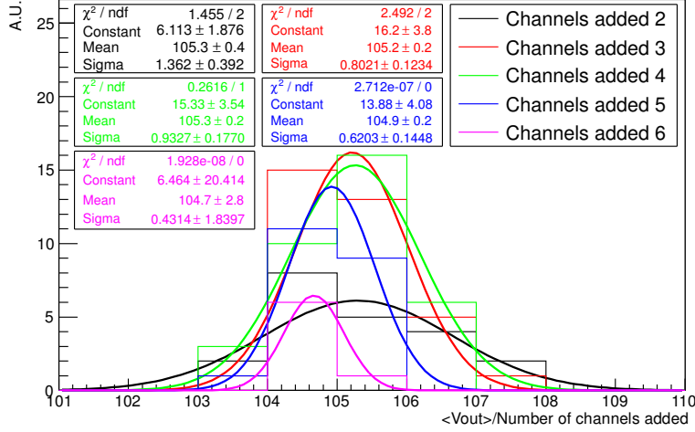
Figure 3.20: Output of the majority adder divided by the number of channels added. Histograms for the different number of channels added are shown in different colors (2 channels in black; 3 channels in red; 4 channels in green; 5 channels in blue; 6 channels in magenta) and fit with a gaussian, represented by a line of the same color as the histogram. The results of the fit are shown in the plot with the same color as the fit. Constant corresponds to A , Mean to \mu and Sigma to \sigma as they are expressed in equation 3.1.
