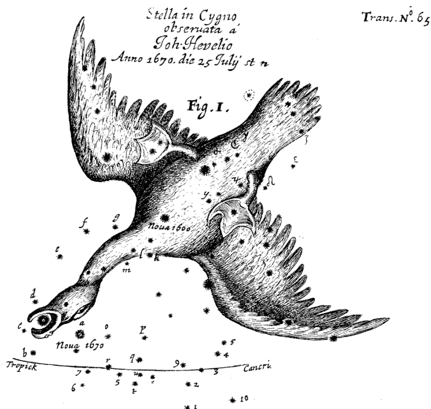
Figure 8.2: Chart of the nova Vulpeculae (tagged as “nova 1670”), the first nova identified by European astronomers (Hevelius 1670). The star tagged as “Nova 1600” was believed to be a nova, but is currently known as P Cygni, an hypergiant luminous blue variable whose brightness variations are attributed to the ejection of its outer layers.
