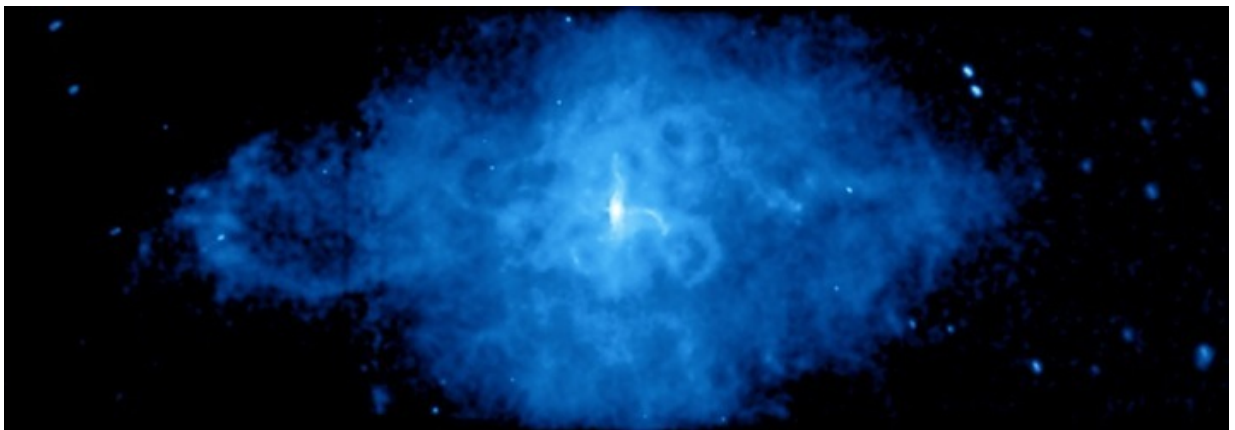
Figure III: Chandra image of 3C 58.
