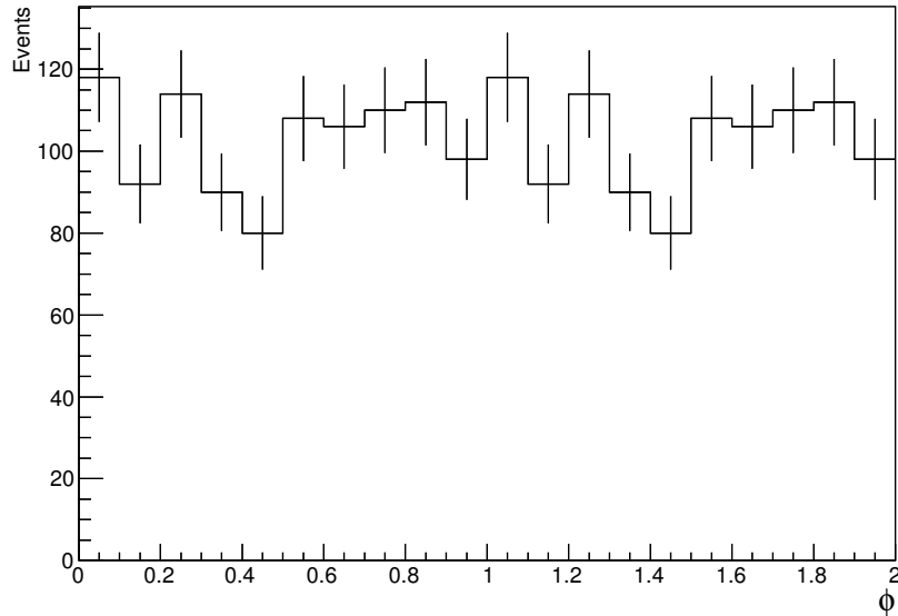
Figure 7.5: PSR J0205+6449 phaseogram above 420 GeV. Two periods are shown for clarity.
