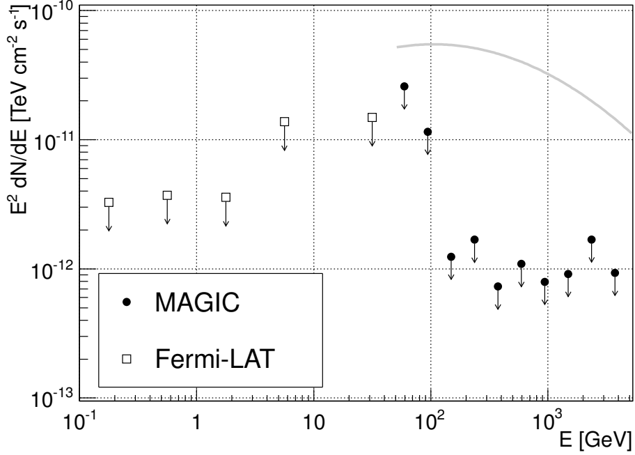
Figure 10.5: Differential ULs on the flux from ASASSN-13ax measured by MAGIC (filled circles) and Fermi -LAT (empty squares). For comparison a spectrum of Crab Nebula is shown with a grey curve.
