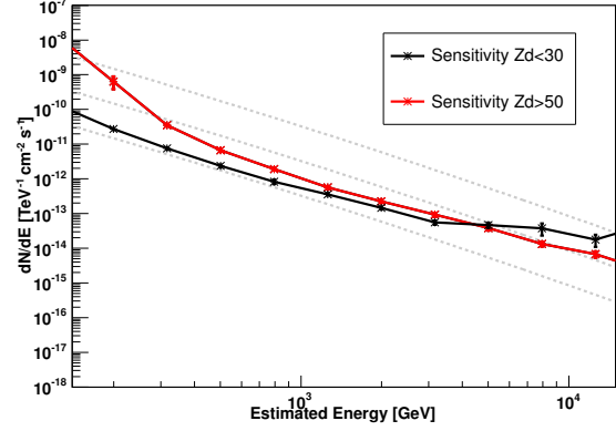
Figure 6.8: MAGIC differential sensitivity for Zd > 50° (red points) and Zd < 30° (black points).
