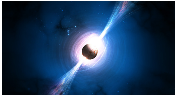
Figure 5.3: Artist view of a pulsar.
