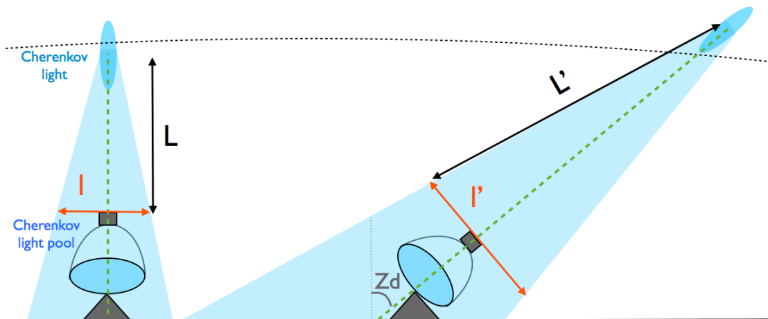
Figure 2.10: Difference in the shower development between low Z_d (left telescope) and high Z_d (right telescope) observations. We can see that the distance from the camera to the point in the atmosphere where the showers start to develop is smaller for low Z_d observation ( L ) than for high Z_d observations ( L' ). The diameter of the Cherenkov light pool in the plane perpendicular to the reflector is also larger for high Z_d observations ( l' \approx l / \cos(Z_d) ).
