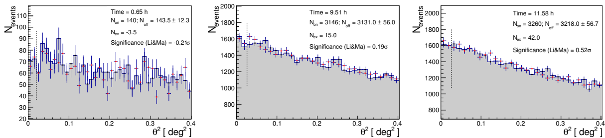
Figure 10.1: Distribution of the squared distance between the nominal and reconstructed source position (red points) and the background estimation (shaded region) in the MAGIC observations of the three objects: YY Her (left panel, E \gtrsim 70 GeV), ASASSN-13ax (middle panel, E \gtrsim 110 GeV) and V339 Del (right panel, E \gtrsim 80 GeV).
