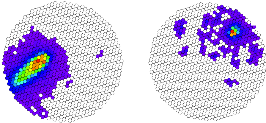
Figure 2.9: Example of an image of a \gamma -ray (left panel) and hadron (right panel) showers.
